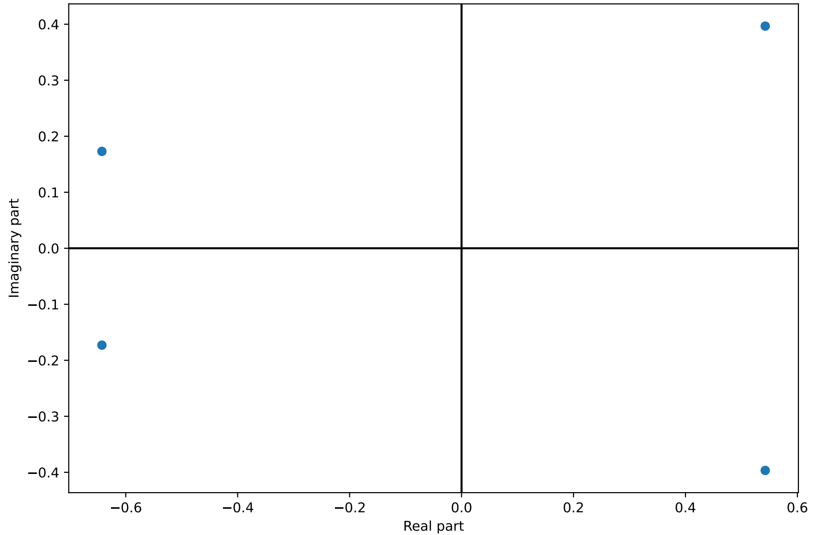
Polynomial roots
